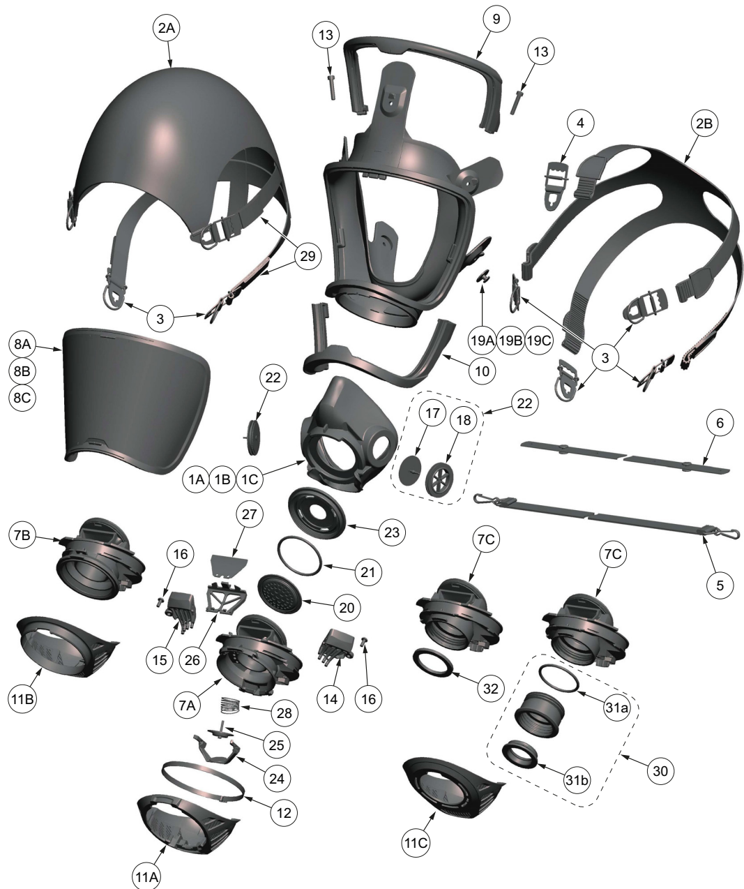
Fig. 14 Exploded View
