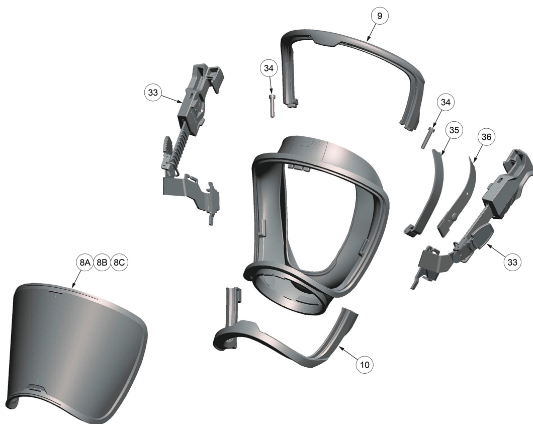
Fig. 15 Mask Helmet Combination - Exploded View
